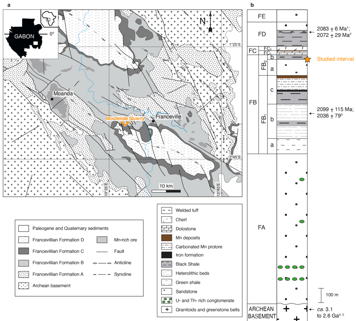
Fig. 1. Geological map of the Paleoproterozoic Franceville sub-basin modified from Bouton et al. (2009a) (a) and general lithostratigraphic column of the Francevillian Group (b). The Moulendé Quarry is the studied area. Sources of ages: 1 - Horie et al. (2005); 2 - Thiéblemont et al. (2009); 3 - Bros et al. (1992); 4 - Moulié et al. (2014); 5 - Ossa Ossa et al. (2020). The figure is modified from Aubineau et al. (2020).
