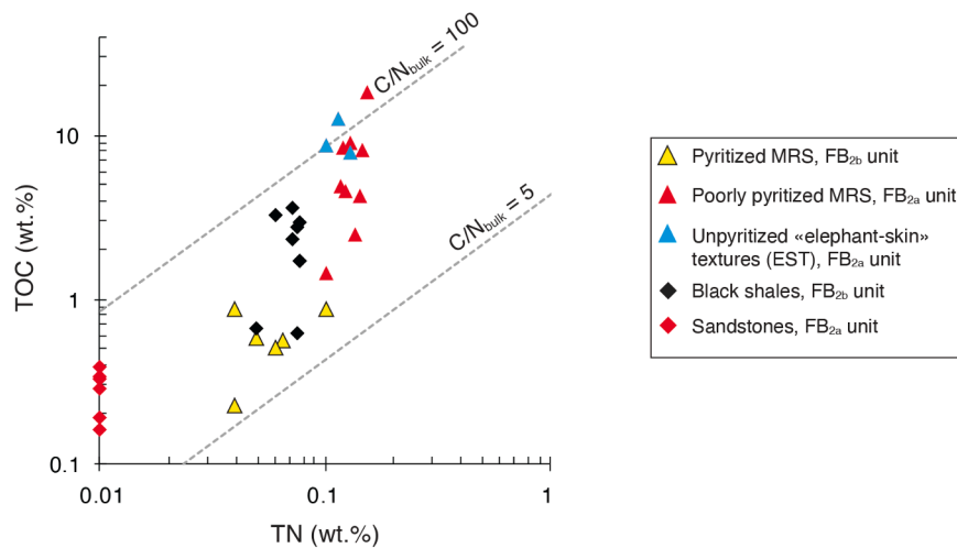
Fig. 6. Cross plot of total organic carbon versus total nitrogen for MRS and host sediments. Dotted lines show molar C:N ratios of 5 and 100. The molar C:N values of modern marine phytoplankton range from 4 to 10 (Ader et al., 2016; Canfield et al., 2010). Remineralization of biomass in the water column and during diagenesis increases the C:N ratios.
