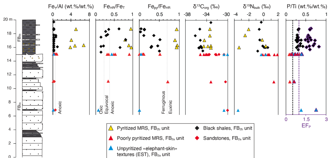
Fig. 3. Geochemical data for the MRS and host sediments plotted along the lithostratigraphic profile of the studied sequence of the FB 2 Member. Grey, black, and purple vertical lines represent redox boundaries as in Raiswell et al. (2018), the UCC value from Rudnick and Gao (2003), and the EF P for the UCC is 1, respectively. Fe/Al for the UCC is shown with grey dash line.
