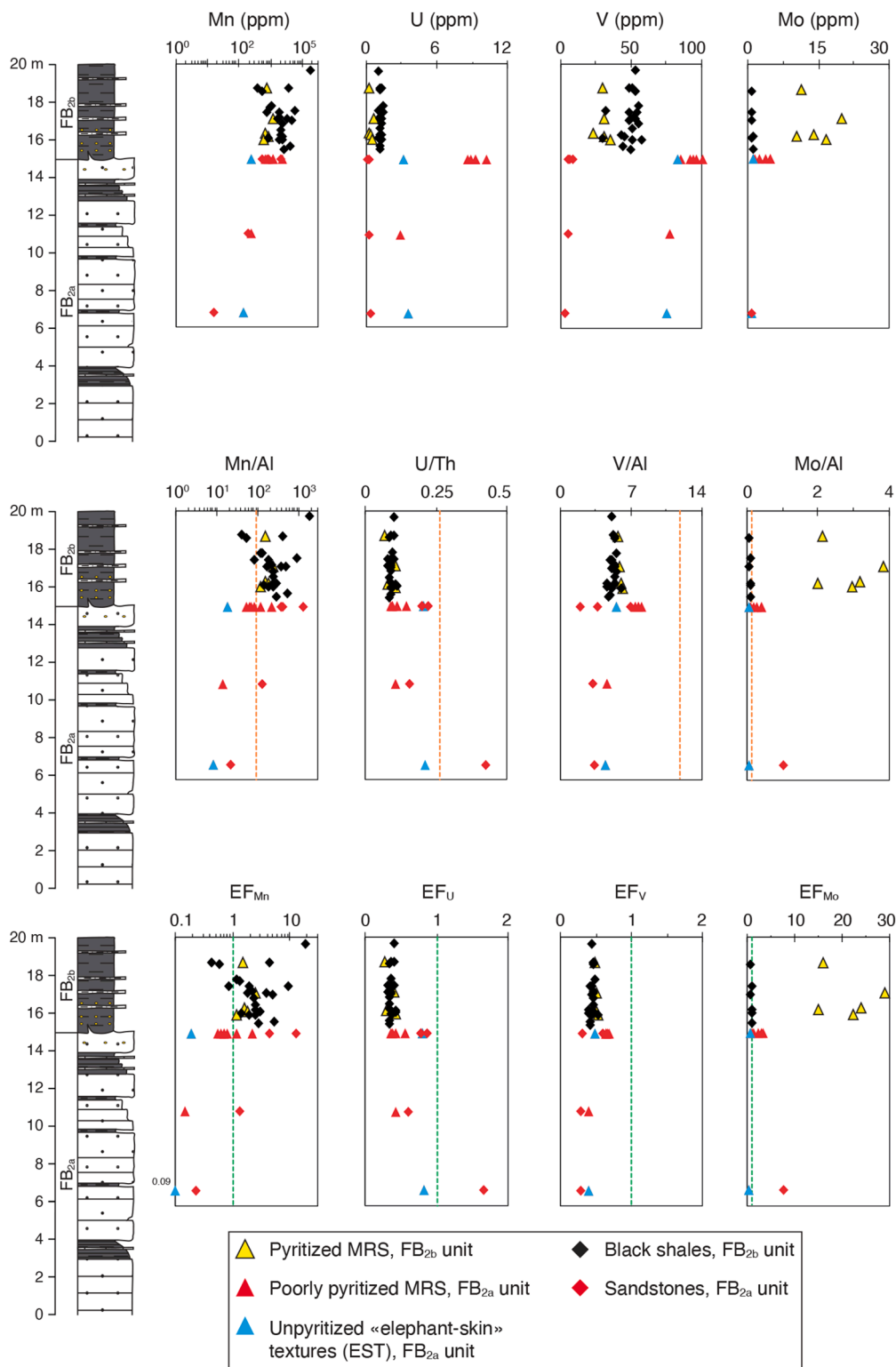
Fig. 4. Data for redox-sensitive metals from the MRS and host sediments plotted along the lithostratigraphic profile of the studied sequence of the FB 2 Member. Orange and green vertical lines correspond to the UCC ratio from Rudnick and Gao (2003) and the EF for the UCC of 1, respectively. The Mn/Al, V/Al, and Mo/Al ratios are expressed in ppm/wt.%.
